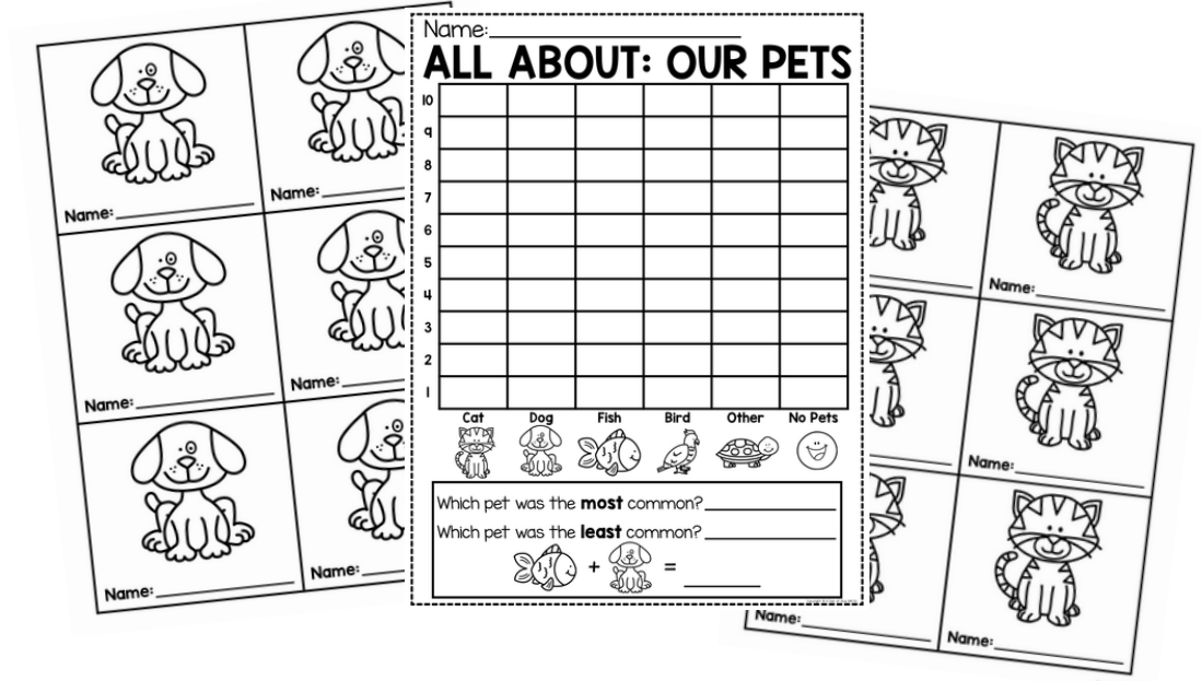
class graph
